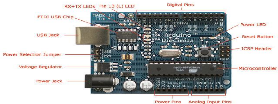
Figure 1: Arduino Circuit
